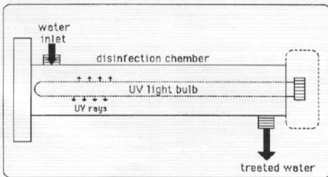
Figure 1. Cross sectional diagram of typical UV disinfection unit.
